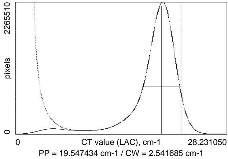
030208a (25 keV, 1.5 sec.) / rutile #55-2
