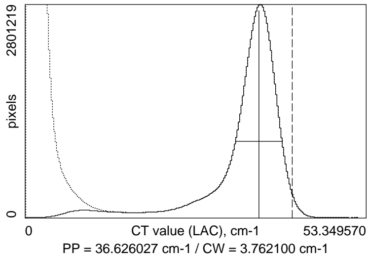
030208b (20 keV, 2 sec.) / rutile #55-2
